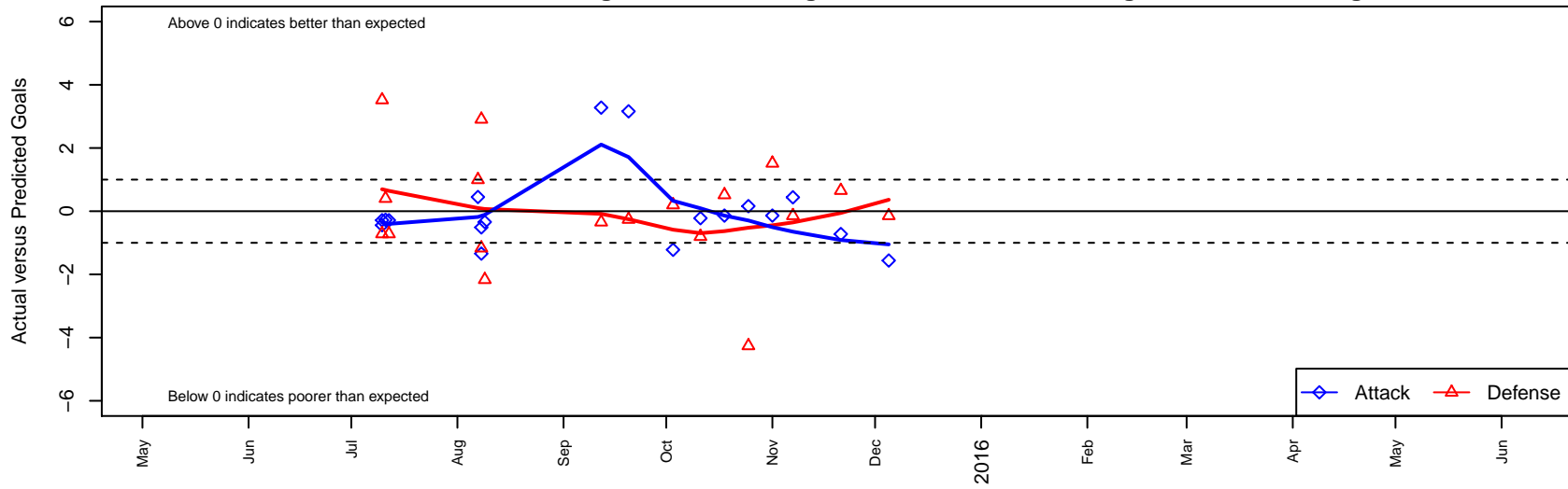
FWFC Tsunami B99 Dots are actual minus expected GF (blue circles) and GA (red triangles). Blue line is smoothed change in attack strength. Red is smoothed change in defense strength.
